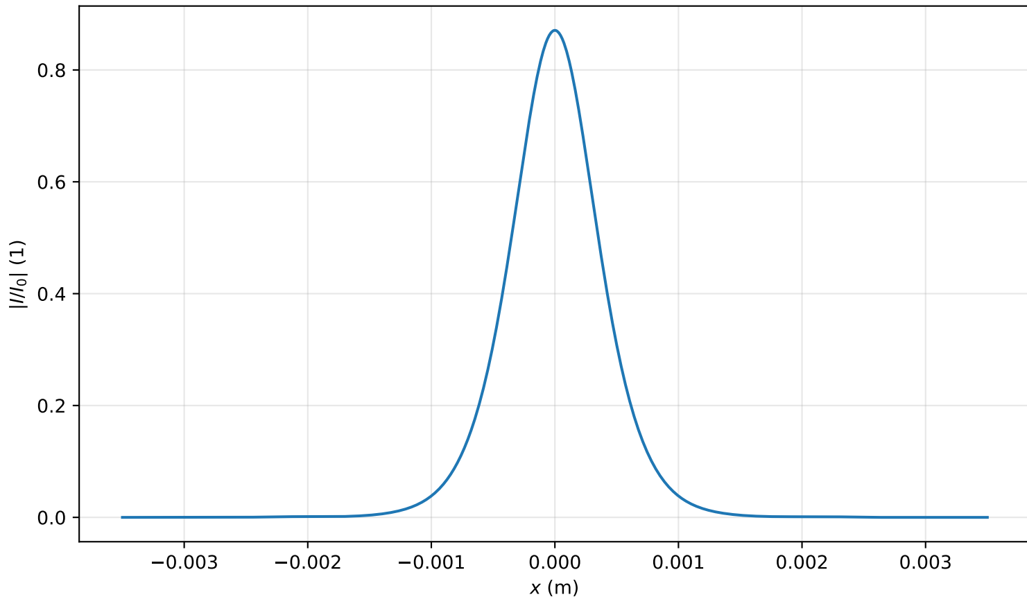
Intensity profile I(x, y = 0, z = 3.981m)/I_0 , P_{in}=0.8P_{cr} , artificial time
